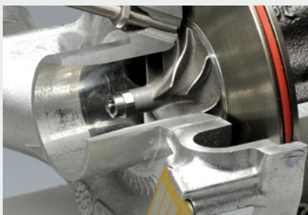
Rotational speed measurement of turbochargers
